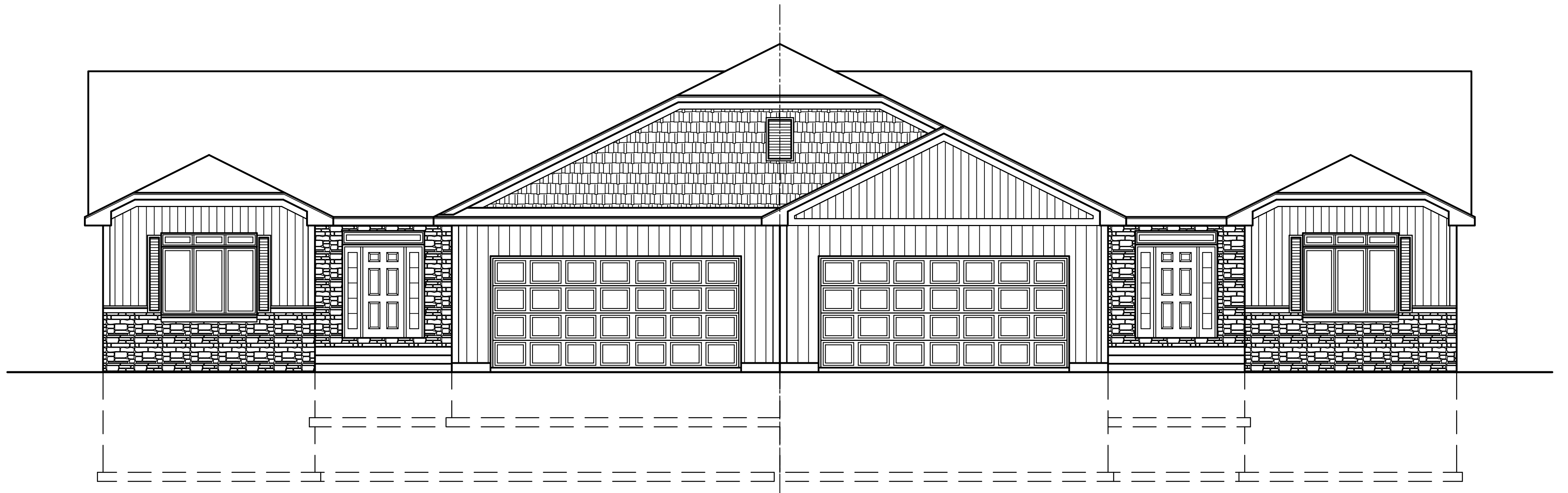
FRONT ELEVATION MEADOW BREEZE 1
