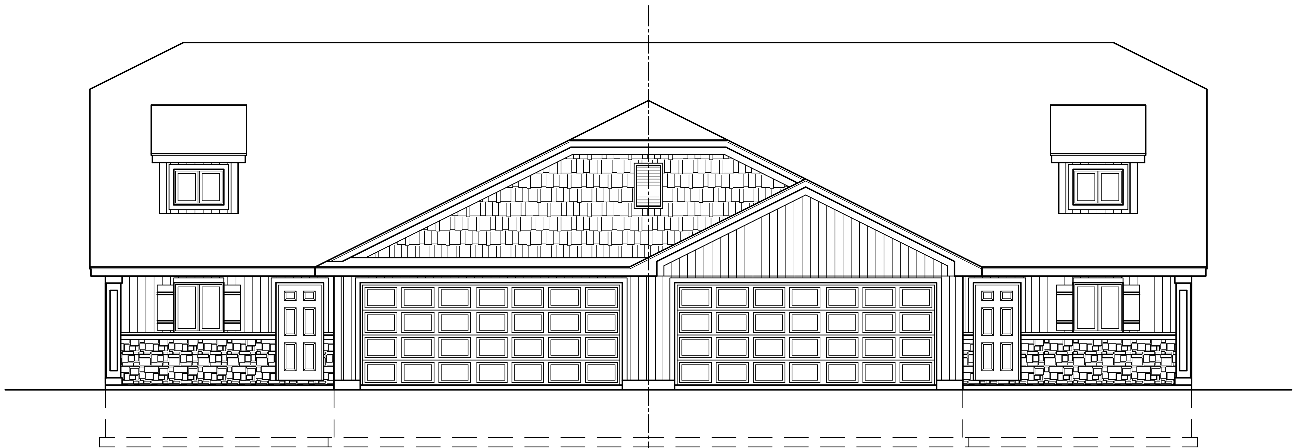
FRONT ELEVATION MEADOW LARK 1
